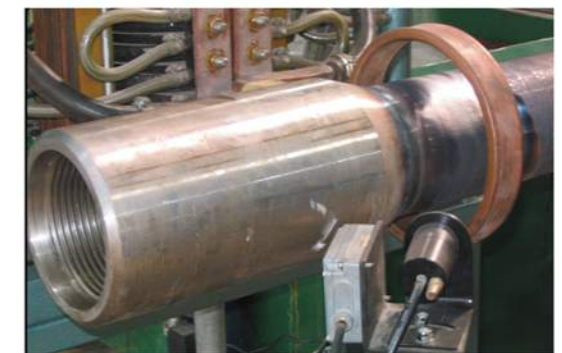
焊缝回火 Weld tempering
